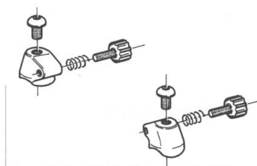
ERGOPOWER BLOCKS FOR STEEL FRAME
