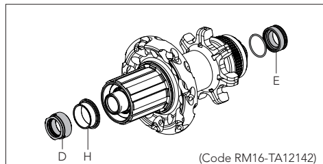
THRU AXLE HH10 - 142 mm
